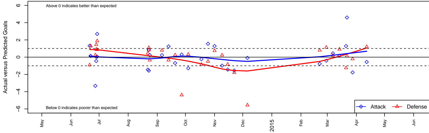
FC Tacoma Blue G01 Dots are actual minus expected GF (blue circles) and GA (red triangles). Blue line is smoothed change in attack strength. Red is smoothed change in defense strength.
